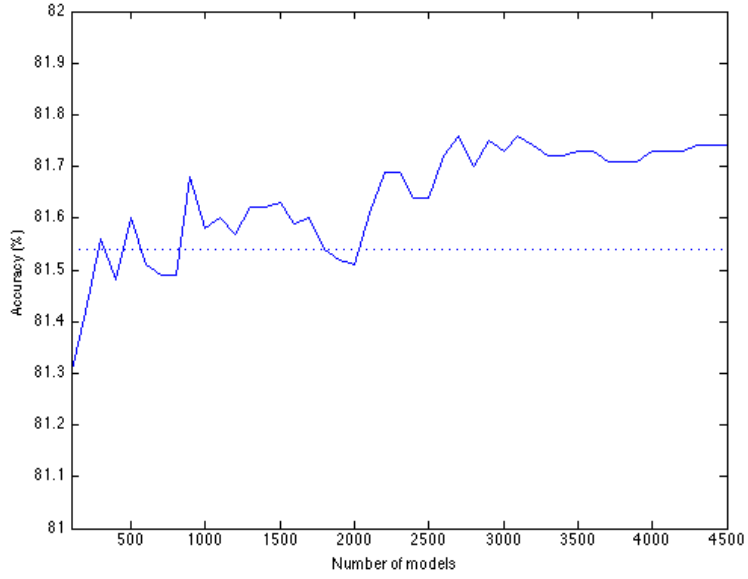
(a) Accuracy-number of sub-models for dropout network
