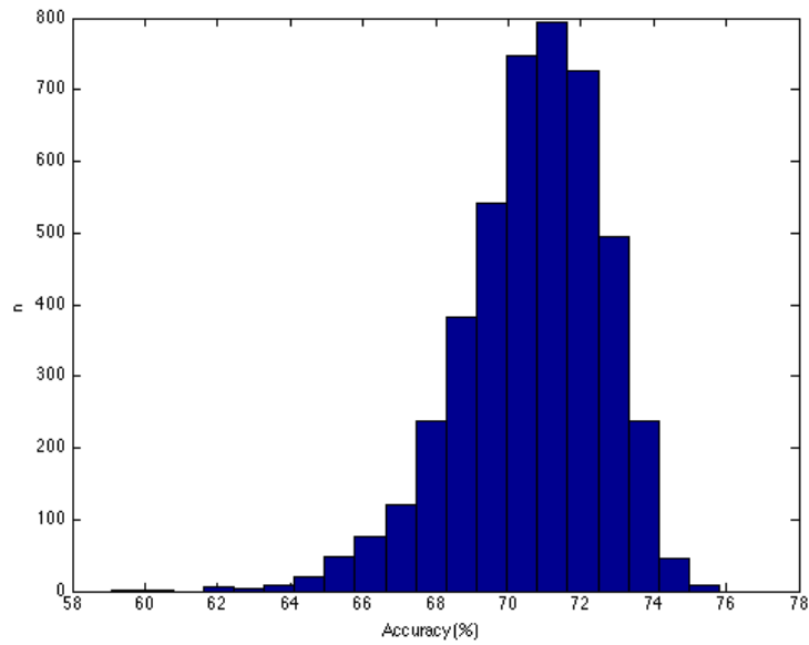
(b) Histogram of accuracies of sub-models of nondropout network
